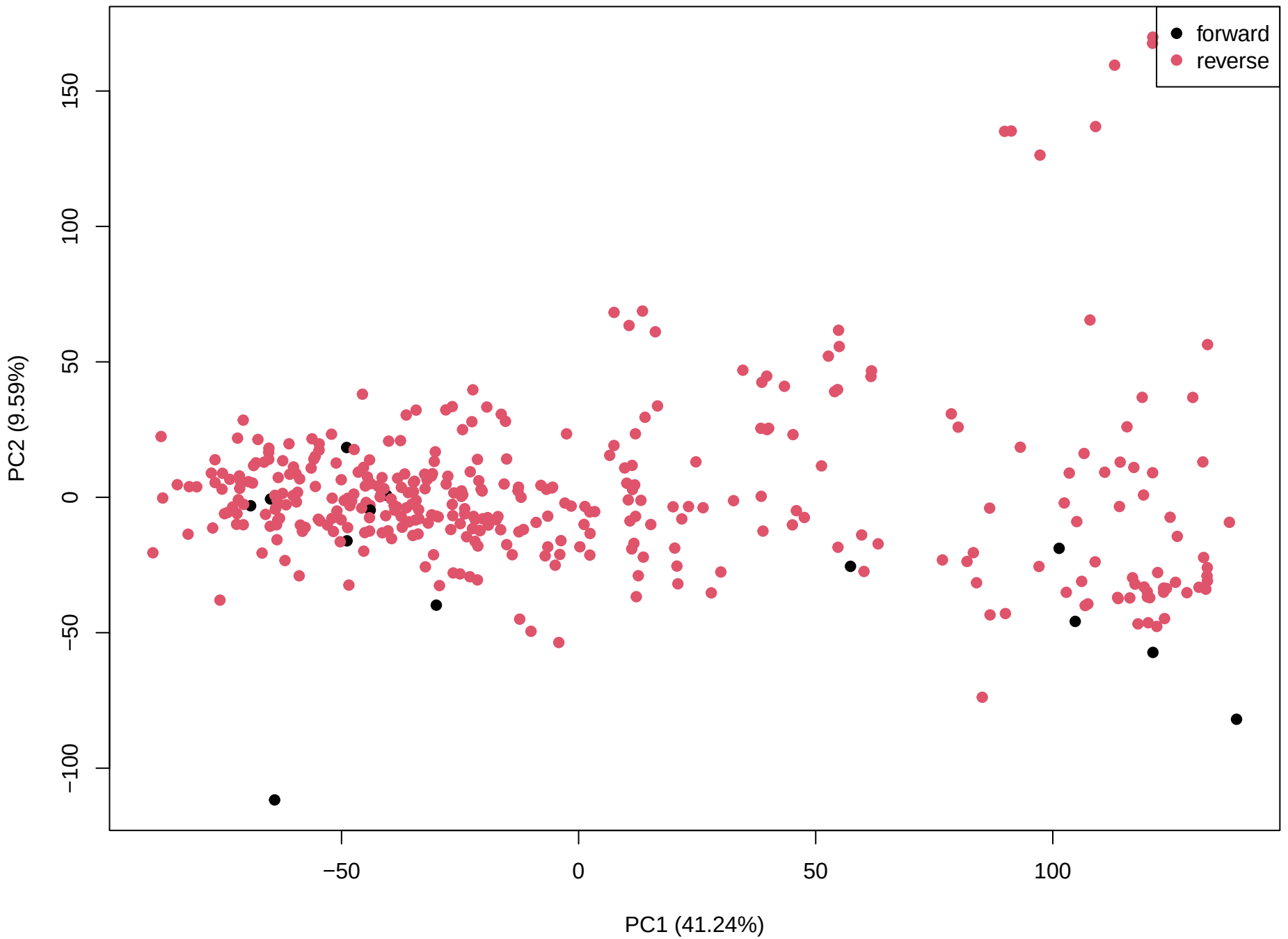
PCA Before Batch Correction
